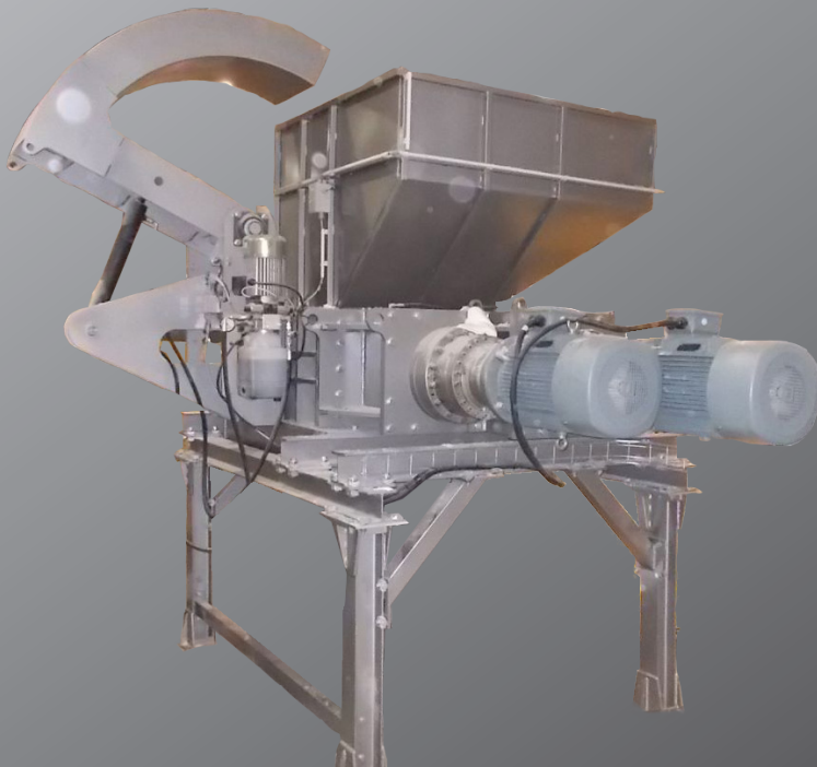
B840-750 with big electric arm (view from front)
